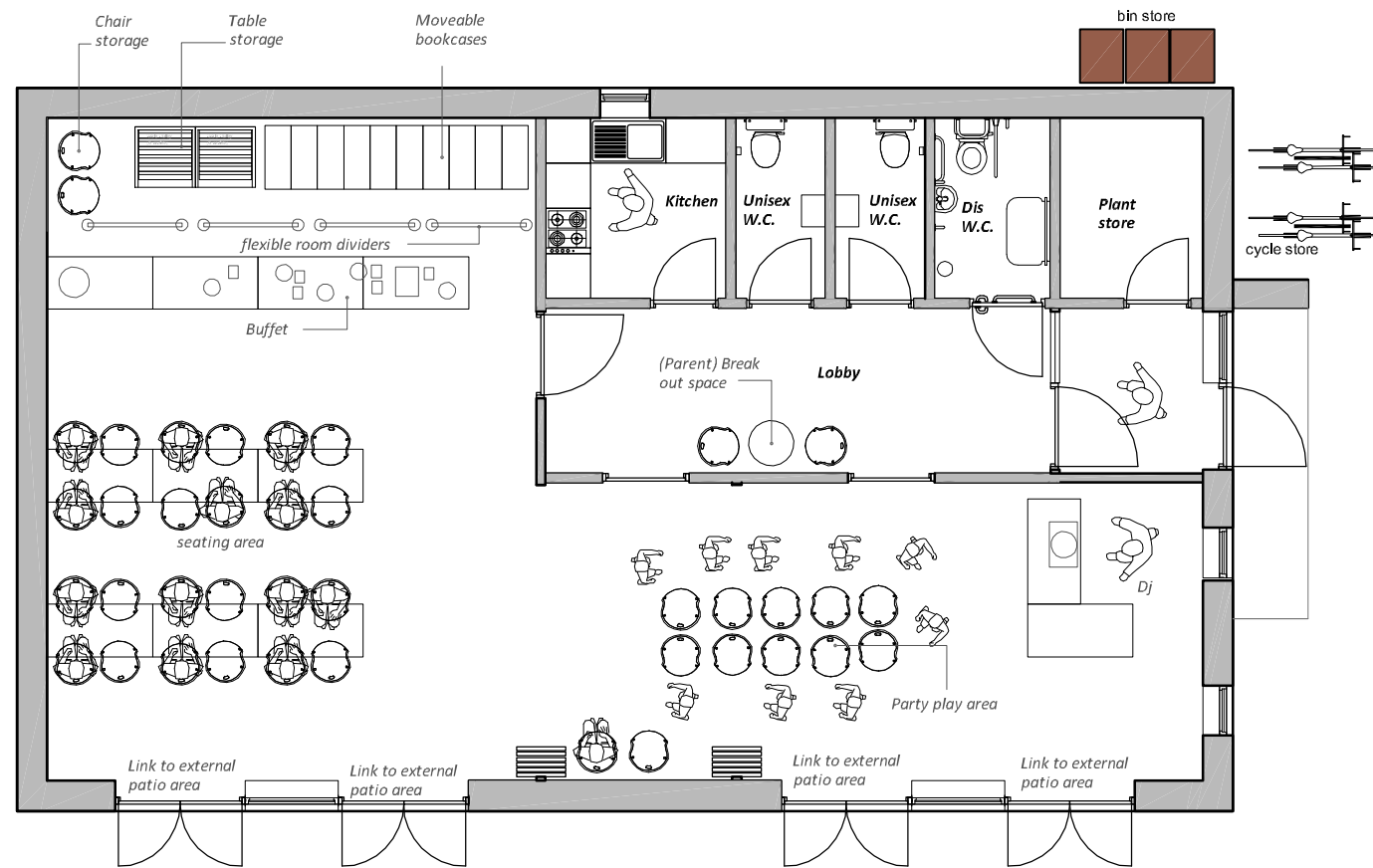
Ground Floor Plan - Single Use
