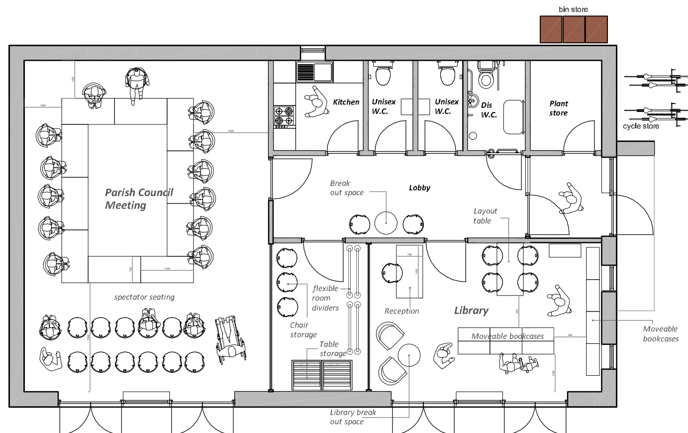
Ground Floor Plan - Multi-use
